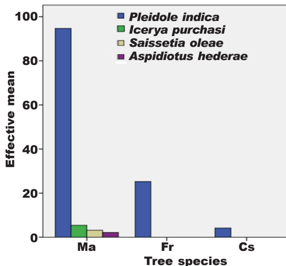
Fig. 3. Fluctuation of the population of Hemipterans species and the ant P. indica in three trees species (Ma, Morus alba ; Fr, Ficus retusa ; Cs, Cupressus sempervirens ).
